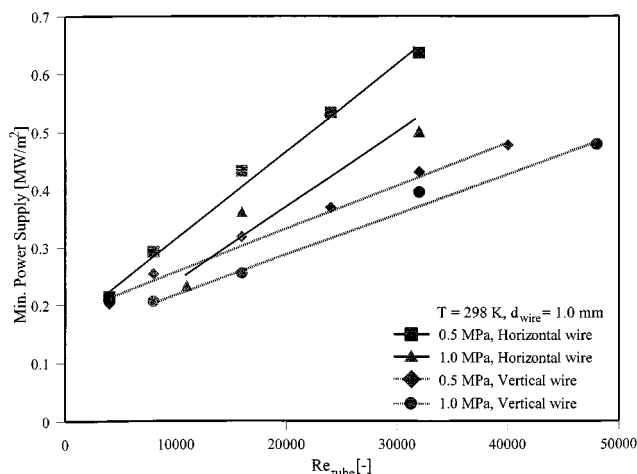
Figure 4. Minimum power supply at ignition, expressed in MW/m^2 wire surface.
